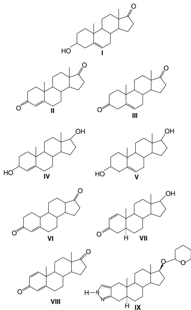
Figure 4 The 'supplements' (I) dehydroepiandrosterone (DHEA), (II) and (III) androstenedione ( \Delta^4 and \Delta^5 versions respectively), (IV) and (V) androstenediol ( \Delta^4 and \Delta^5 versions, respectively), (VI) 19-norandrostenedione (only \Delta^4 version displayed), (VII) 1-testosterone, (VIII) boldione and (IX) prostanzolol.
